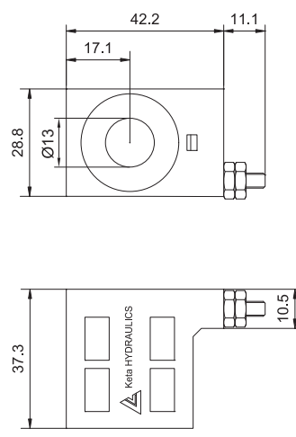
Model:LC2-08-S-*E Single Stud 8-32 Male Stud With 2 Brass Nuts
