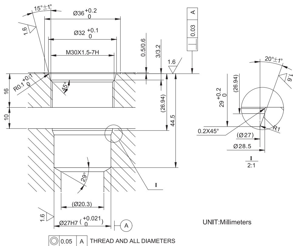
CAVITY: Rexroth-LG
